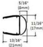
BULB SEAL 1/2"
