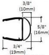
BULB SEAL 3/8" (2 INCLUDED IN KIT)
