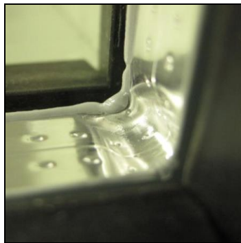
Figure 6 Primary Sealant at Bent Corner
