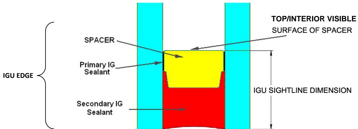
Figure 1 IGU Edge Cross Section
